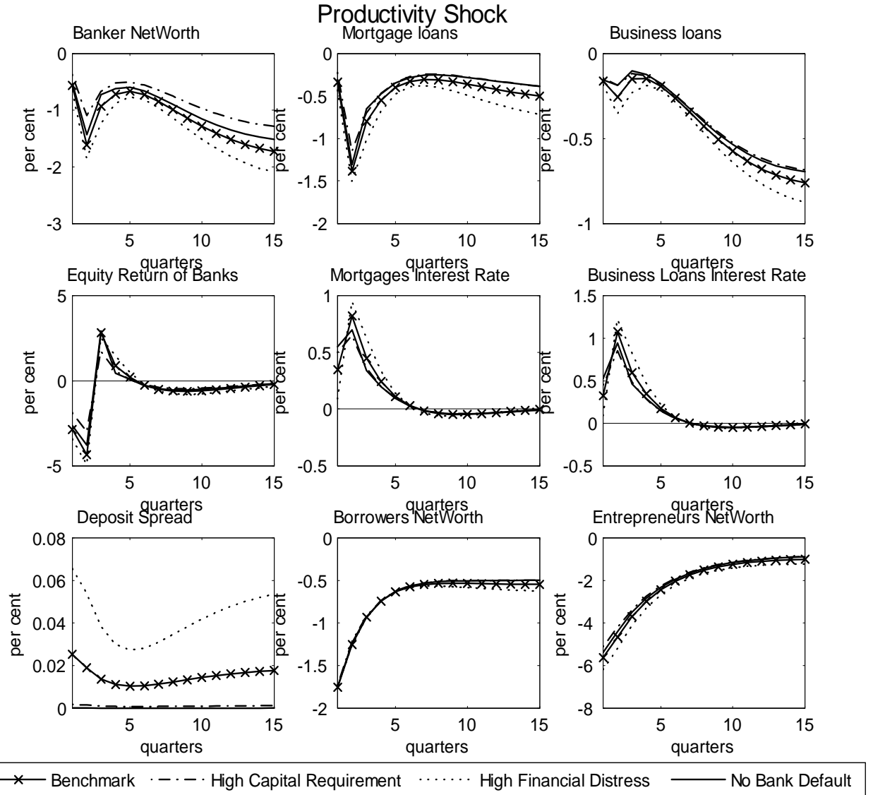
Figure 3c.. Impulse responses after a negative TFP shock (III)
